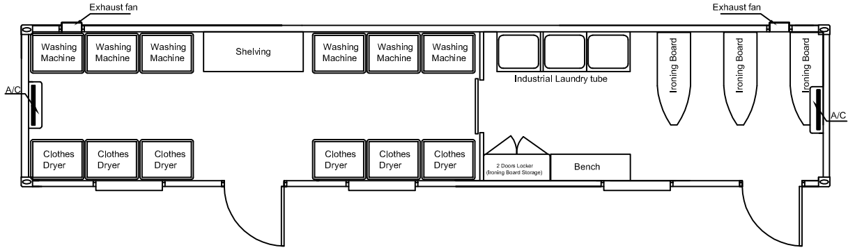
LAY OUT
