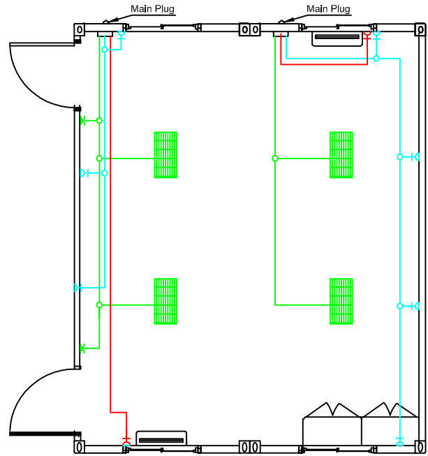
ELECTRICAL INSTALLATION
