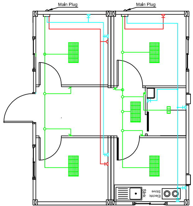
ELECTRICAL INSTALLATION
