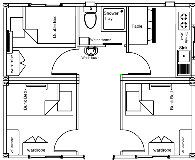
LAY OUT
